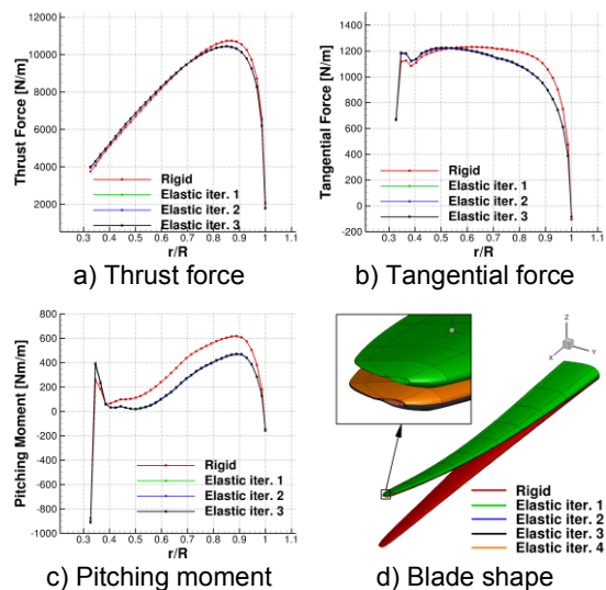
Fig.3 The convergence history of loads and blade shape for static aero-elastic analysis of InnWind blade.
