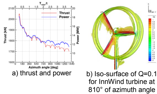
Fig.2 Thrust and power as function of azimuth angle (a) and iso-surface of Q=0.1 at 810° of azimuth angle (b) for the complete InnWind turbine.
