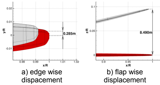
Fig.4 InnWind blade deformation for wind speed of 11m/s. Red – rigid, and grey – elastic blade.
