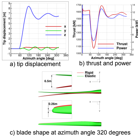
Fig.5 Results of dynamic aero-elastic computation. Tip displacement (a); thrust and power (b) as function of azimuth angle; and (c) the shape of the blade at 320^\circ of azimuth angle.
