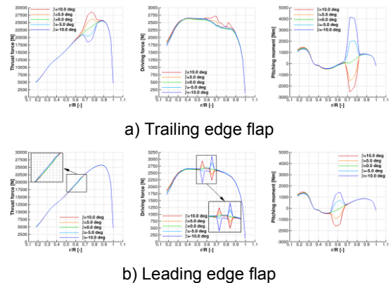
Fig.7 Spanwise distribution of thrust force, driving force and pitching moment for InnWind blade equipped with LE and TE flaps. Flap motion frequency f=0.96 Hz.
