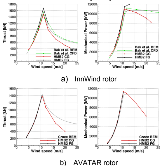
Fig.1 Thrust force and mechanical power as function of wind speed for the InnWind (a) and AVATAR (b) rotors.
