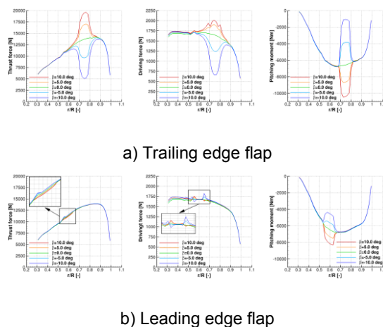
Fig.9 Spanwise distribution of thrust force, driving force and pitching moment for AVATAR blade equipped with LE and TE flaps. Flap motion frequency f=0.16\text{Hz} .
