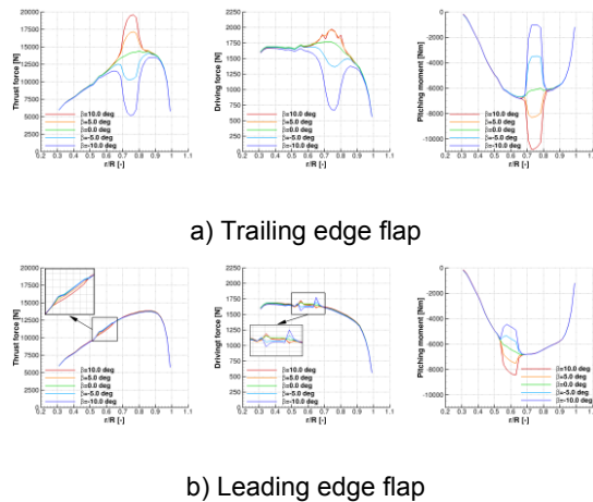
Fig.8 Spanwise distribution of thrust force, driving force and pitching moment for AVATAR blade equipped with LE and TE flaps. Flap motion frequency f=0.96\text{Hz} .
