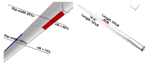
a) the location and dimensions of the trailing and leading edge flaps
